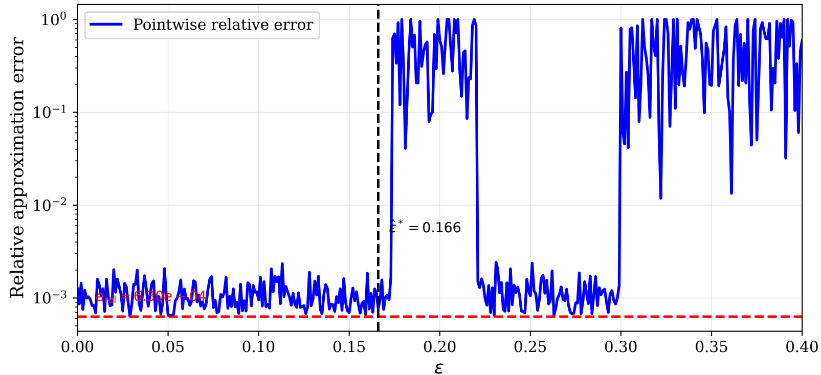
PINN Approximation Error vs \varepsilon
