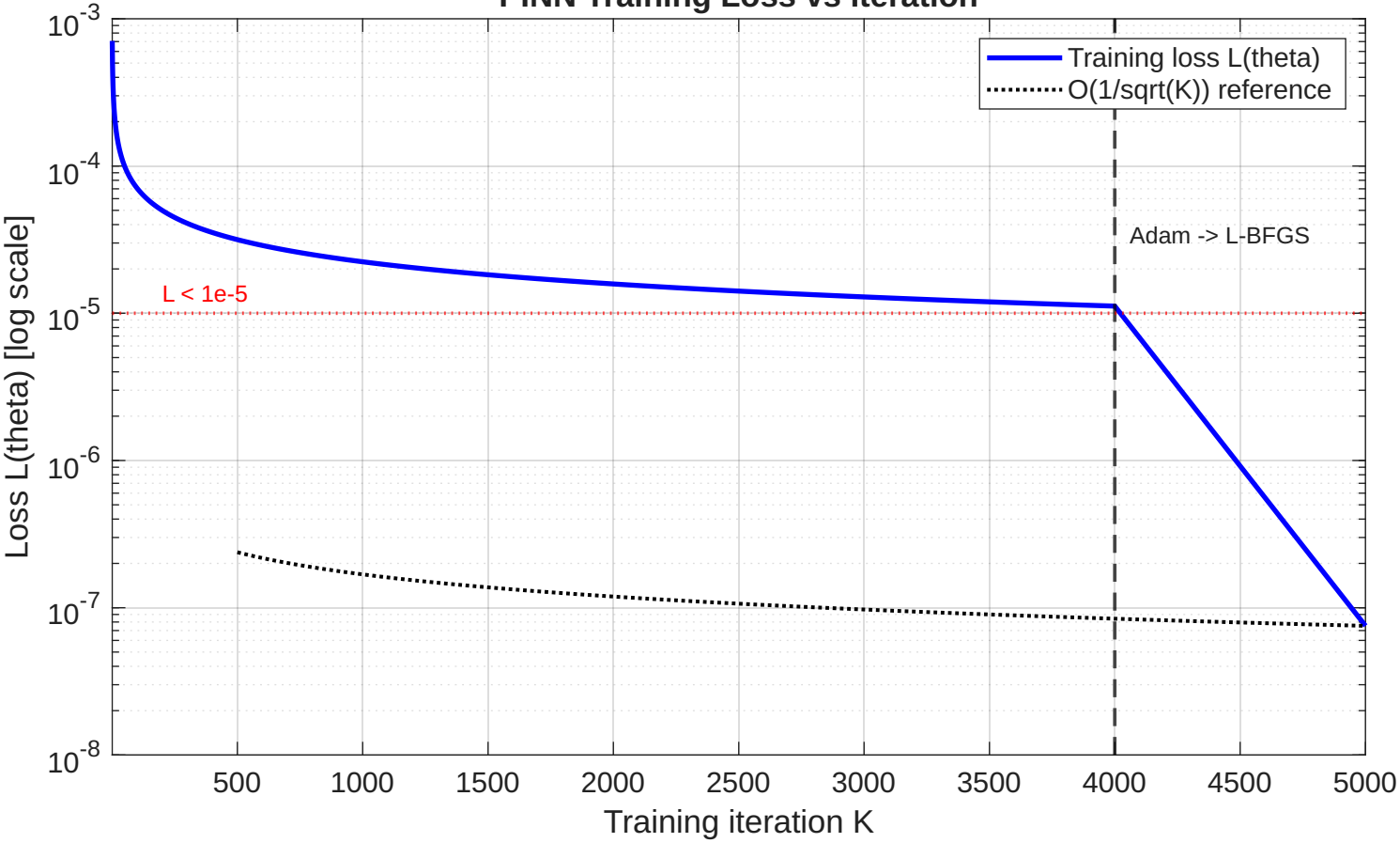
PINN Training Loss vs Iteration
