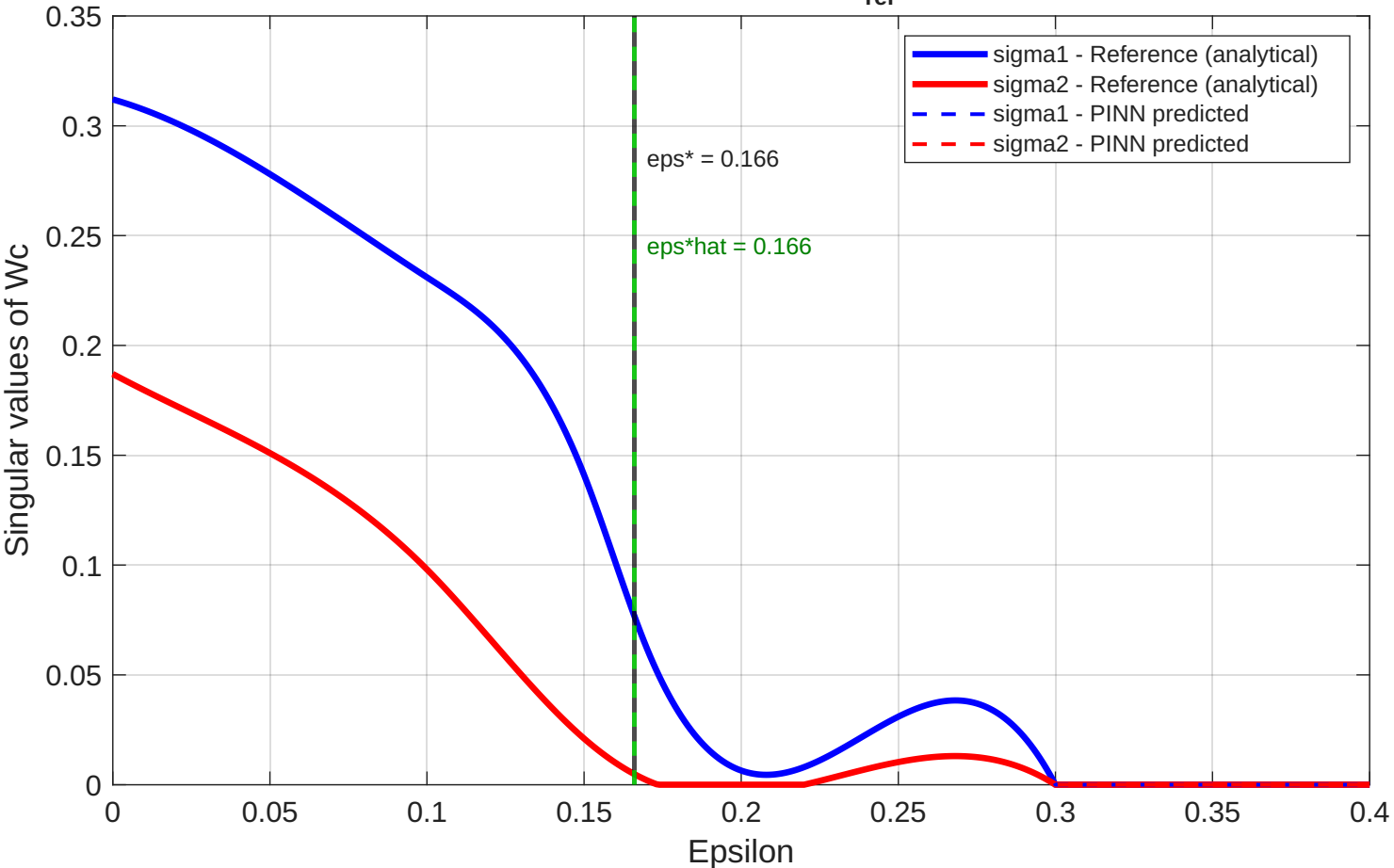
PINN vs Reference Gramian ( e_{rel} = 6.30e-04 )
