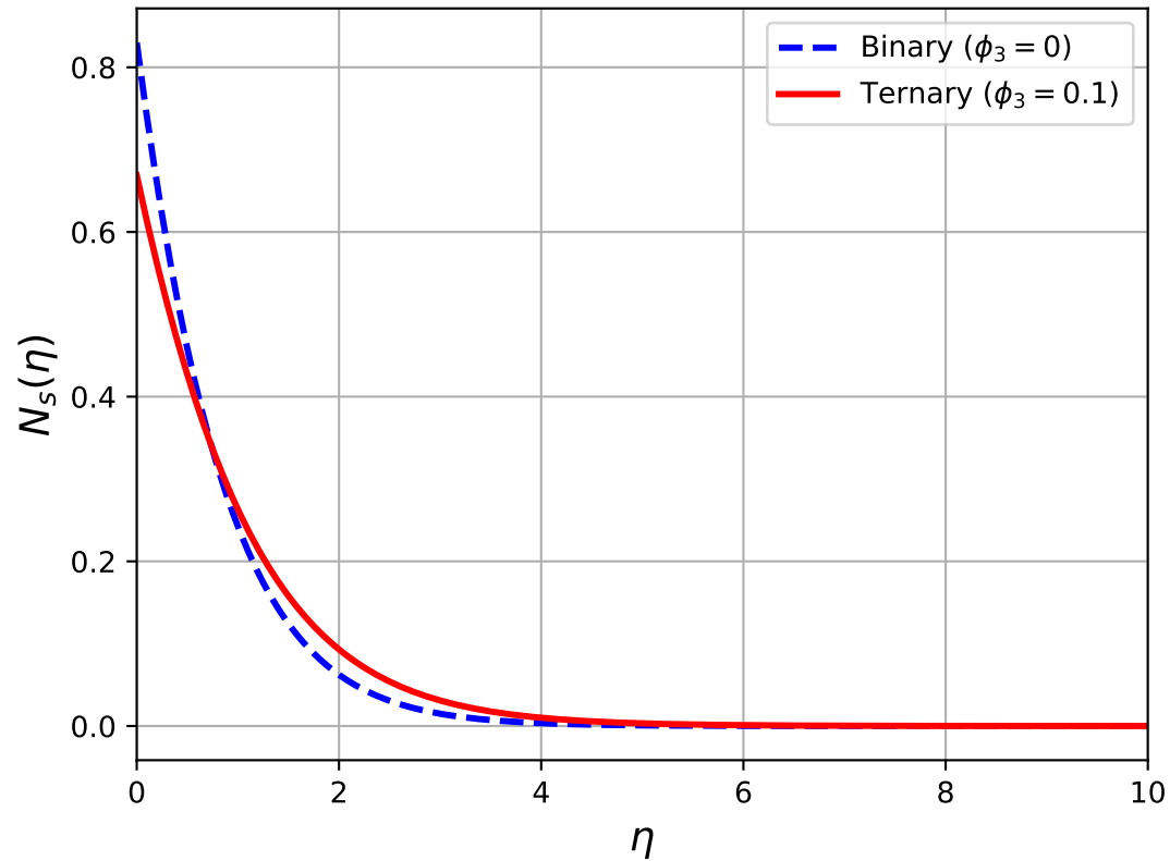
(a) Local entropy generation
