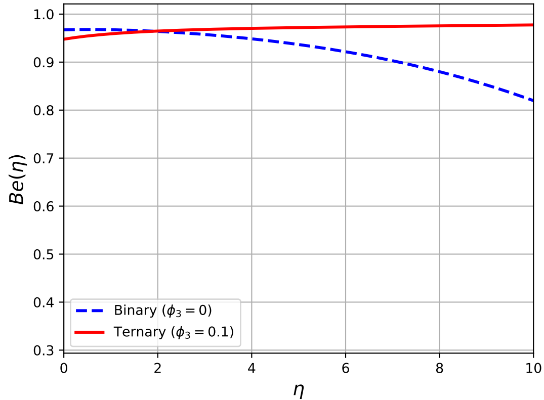
(b) Bejan number
