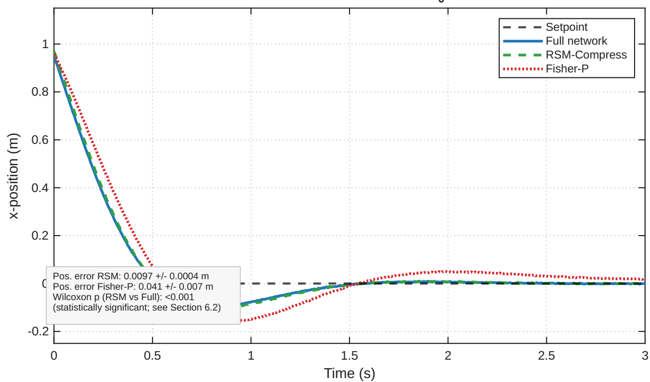
Quadrotor: Representative x-Position Trajectory \epsilon = 0.03 , 2048x compression, x_0 = 1 m
