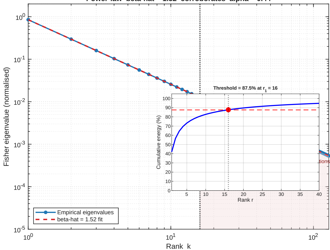
Fisher Eigenvalue Decay (CSTR Layer 1, k = 1 \dots 128 ) Power-law \beta\text{-hat} = 1.52 corroborates \alpha = 0.44
