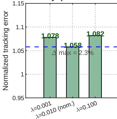
\lambda Sensitivity (1 decade each side)
