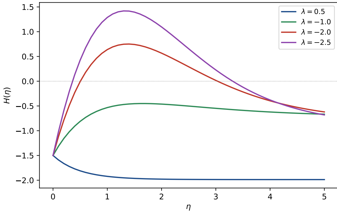
Axial velocity H(\eta) , K = 0.3 , S = 1.5
