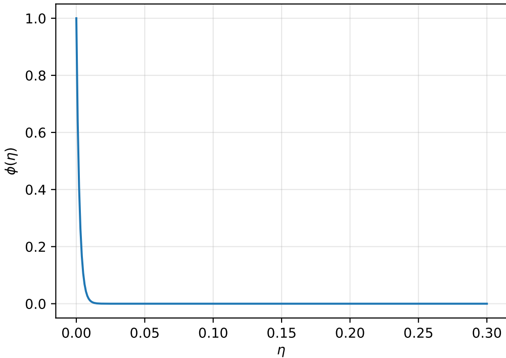
Baseline concentration profile ( Sc \approx 883 )
