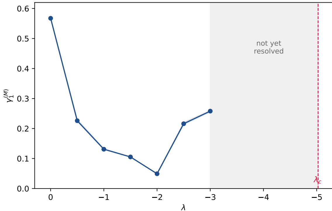
Momentum eigenvalue along the branch, K = 0.3, S = 1.5
