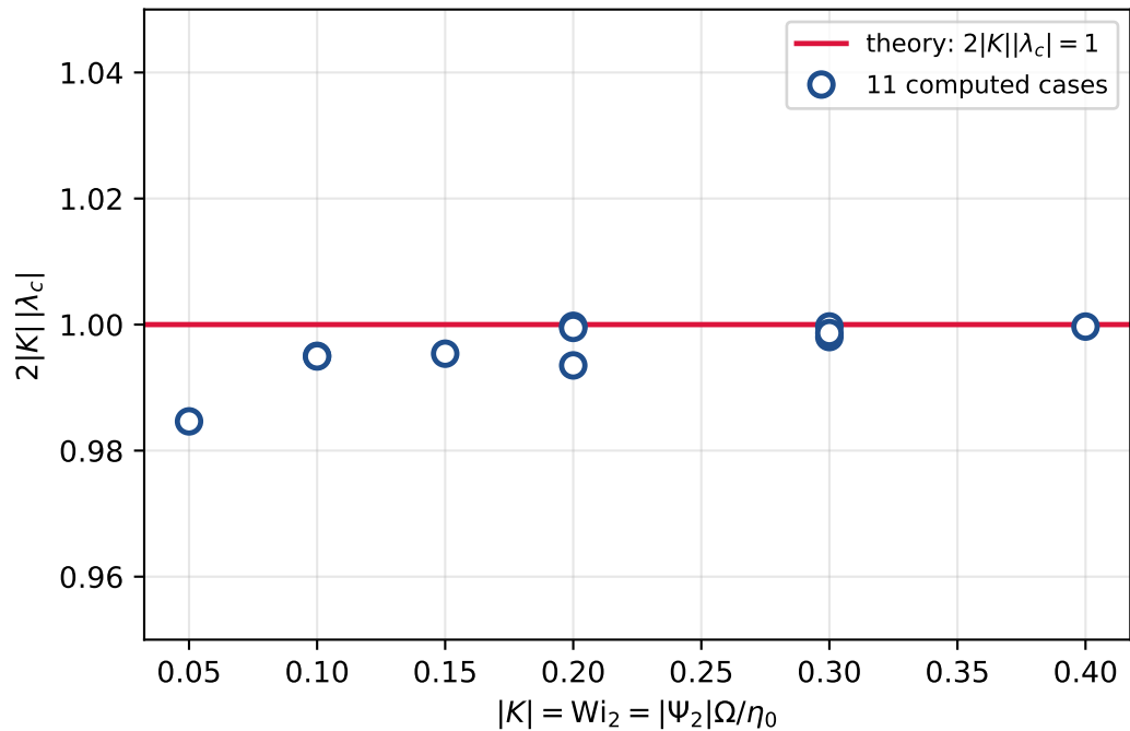
(a) universal collapse
