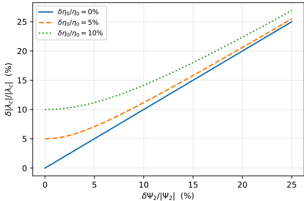
(b) propagated uncertainty in \lambda_c
