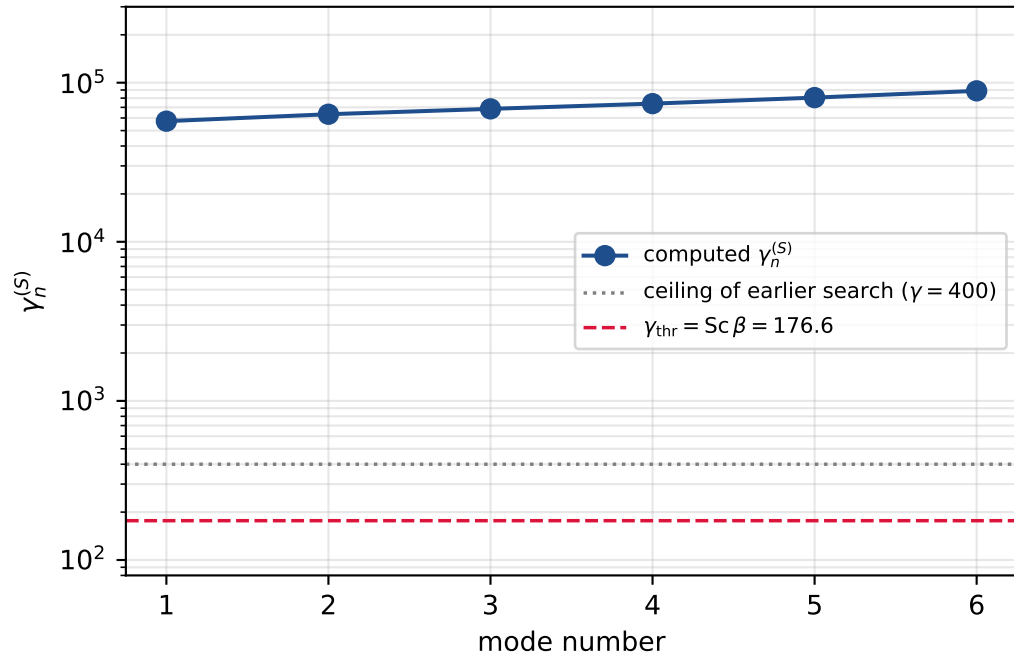
(a) species spectrum: \gamma_1^{(S)} = 5.730 \times 10^4
