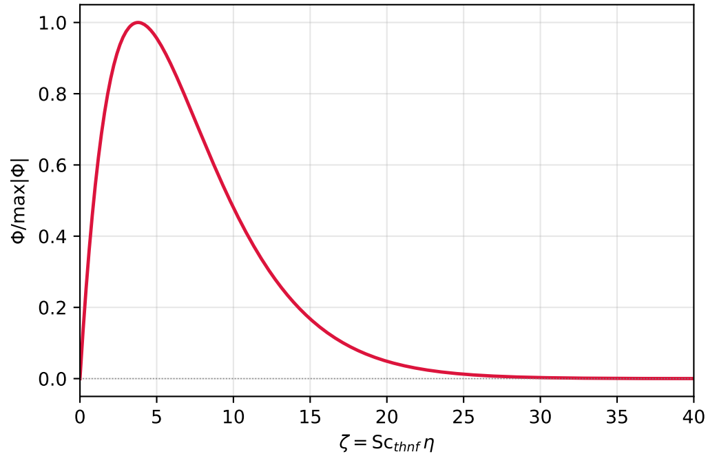
(b) leading eigenfunction in the wall variable
