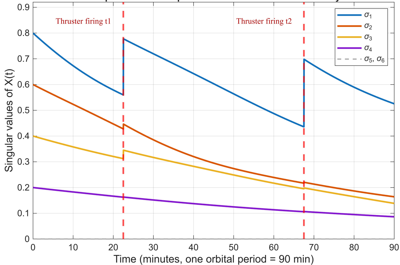
Figure 1: Singular Value Trajectories of Attitude Covariance X(t) Jumps at Thruster Impulse Instants Confirm Rank Recovery
