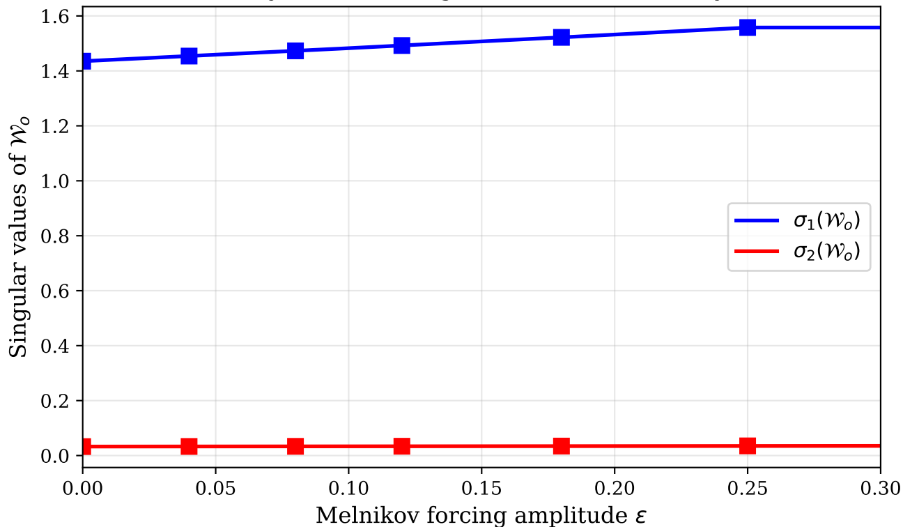
Observability Gramian singular values vs. \varepsilon for system (14)
