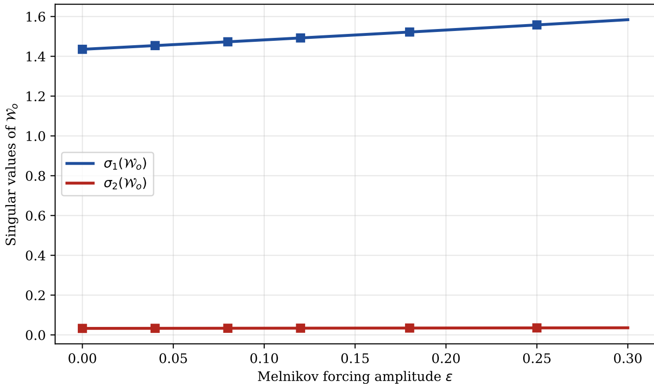
Observability Gramian singular values vs. \varepsilon for eq.~(14)
