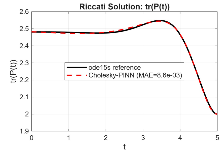
Figure 5 — LQR Riccati: Cholesky-PINN vs ode15s SymErr=0 (algebraic) | MinEig=0.70 | MAE P11 =4.95e-03
