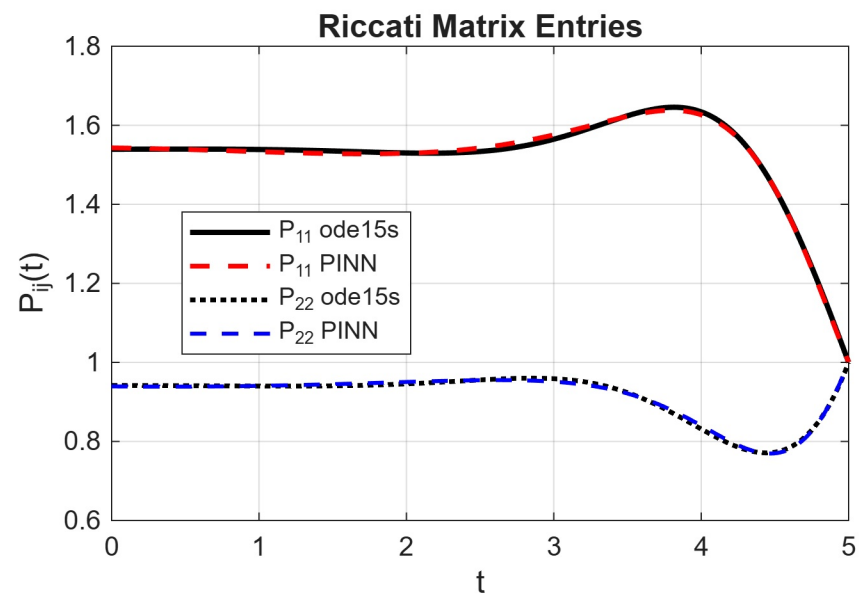
Figure 5 — LQR Riccati: Cholesky-PINN vs ode15s SymErr=0 (algebraic) | MinEig=0.70 | MAE P11 =4.95e-03
