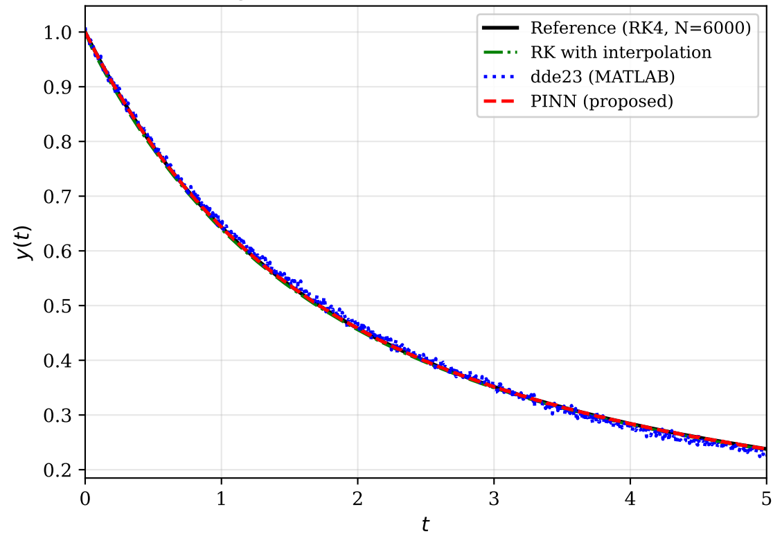
Pantograph DDE: All-Methods Comparison
