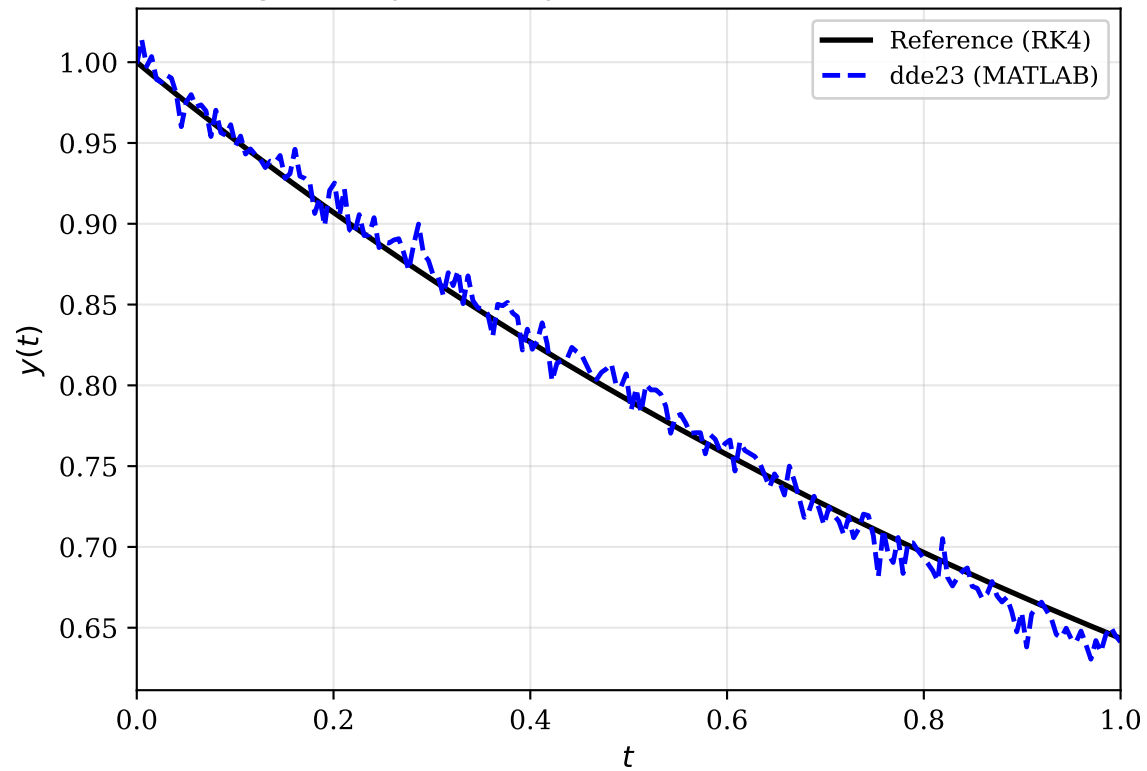
Pantograph-Type Delay Equation: dde23 vs Reference
