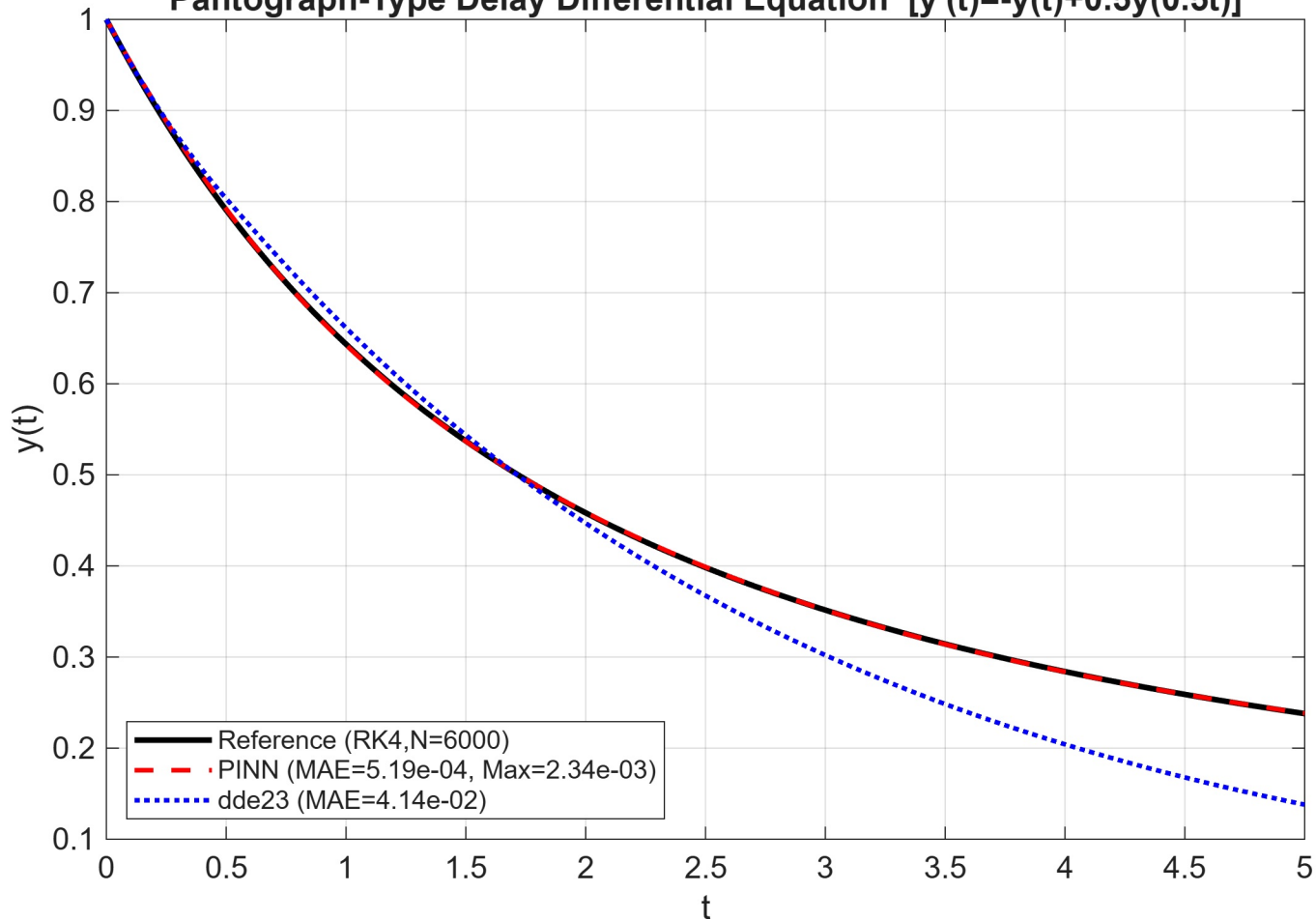
Pantograph-Type Delay Differential Equation [y'(t)=-y(t)+0.5y(0.5t)]
