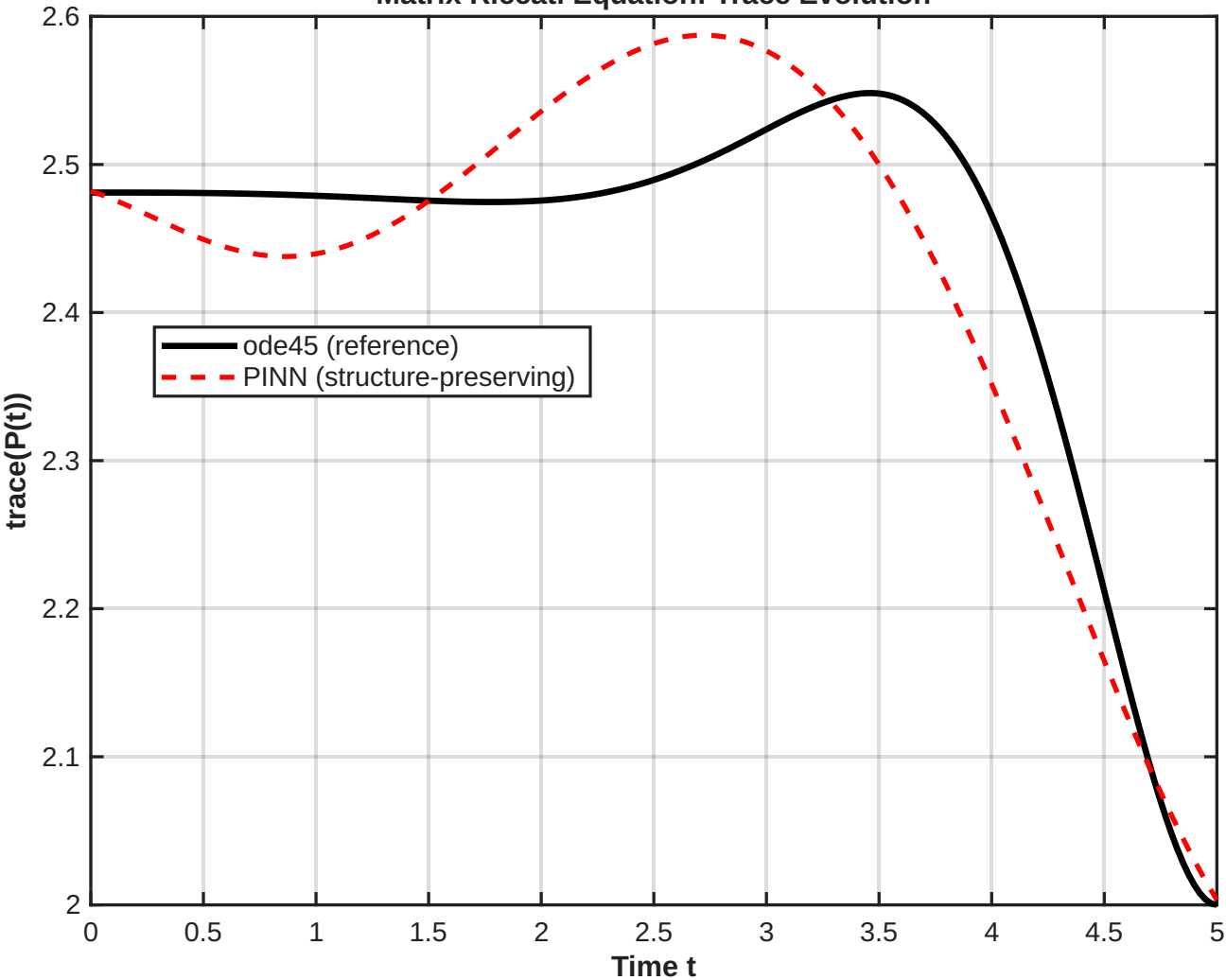
Matrix Riccati Equation: Trace Evolution
