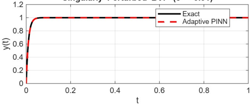
Singularly Perturbed BVP ( \epsilon = 0.01 )
