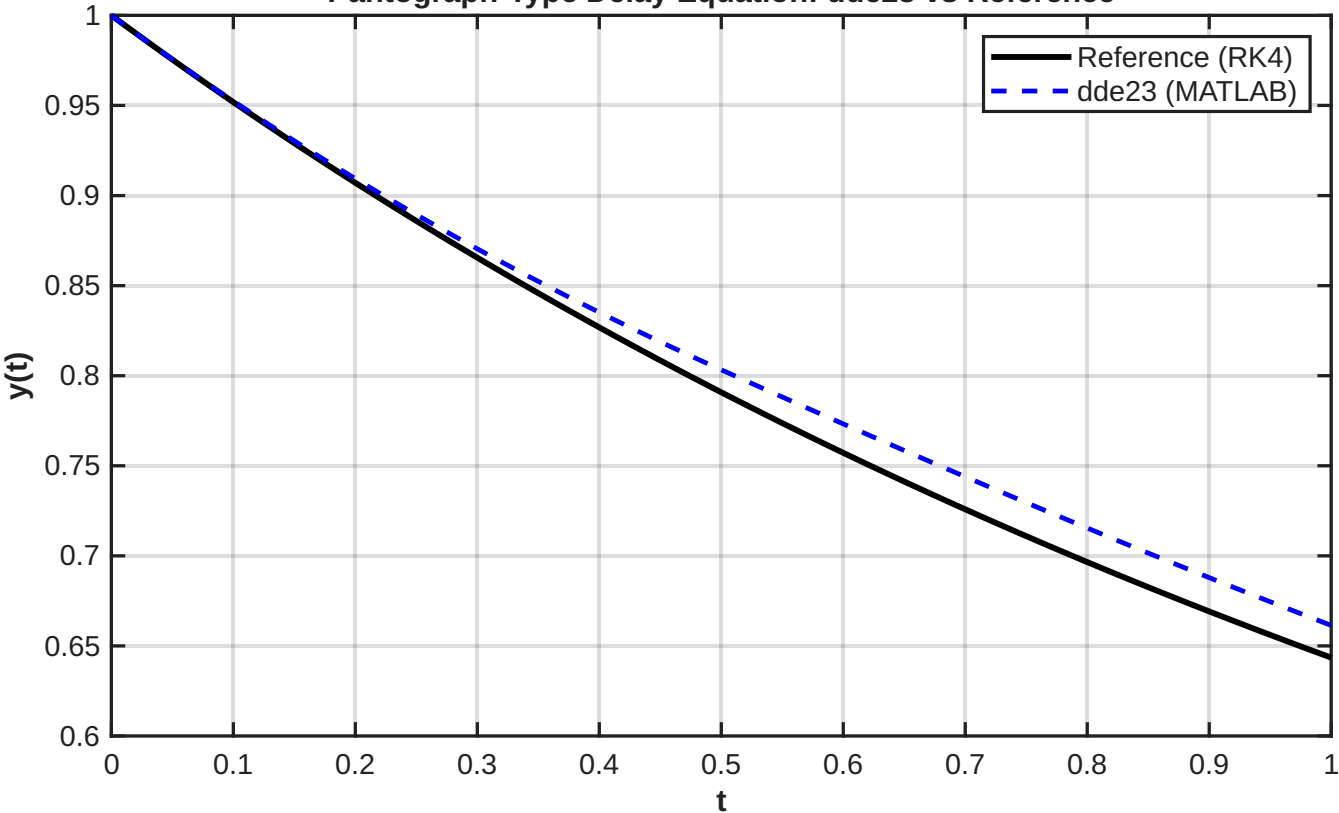
Pantograph-Type Delay Equation: dde23 vs Reference
