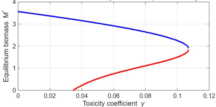
Saddle-node bifurcation (blue = stable, red = saddle)
