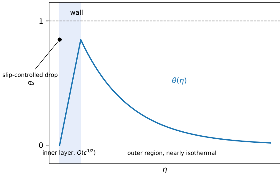
Schematic of the thermal boundary layer at high Pr (not to scale)
