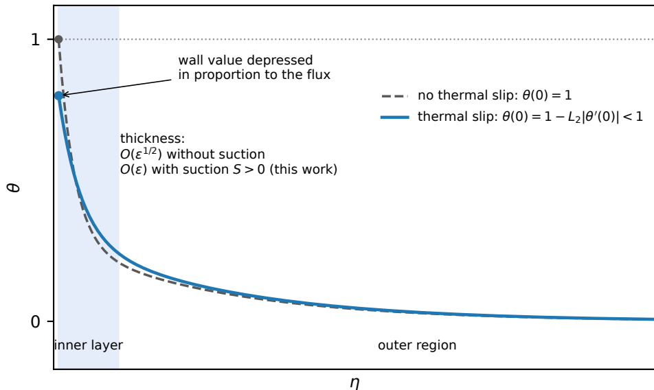
Thermal boundary layer at high Pr, \varepsilon = 1/\text{Pr} (schematic, not to scale)
