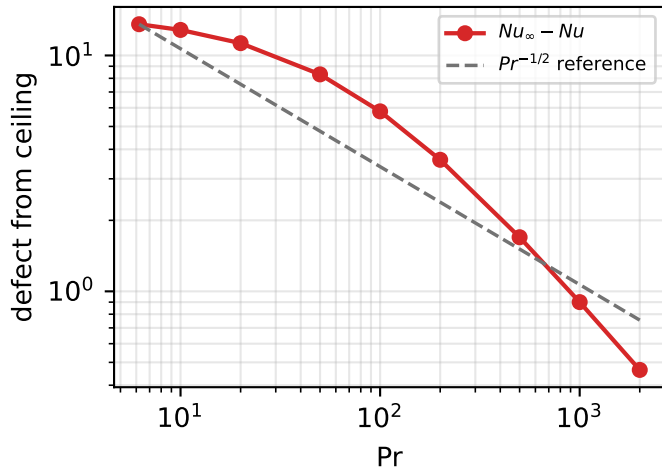
(b) approach to the ceiling
