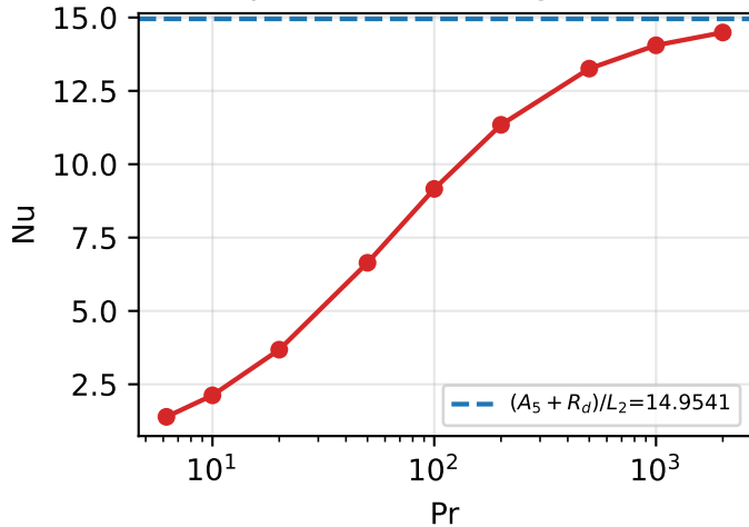
(a) slip-induced ceiling as Pr \rightarrow \infty
