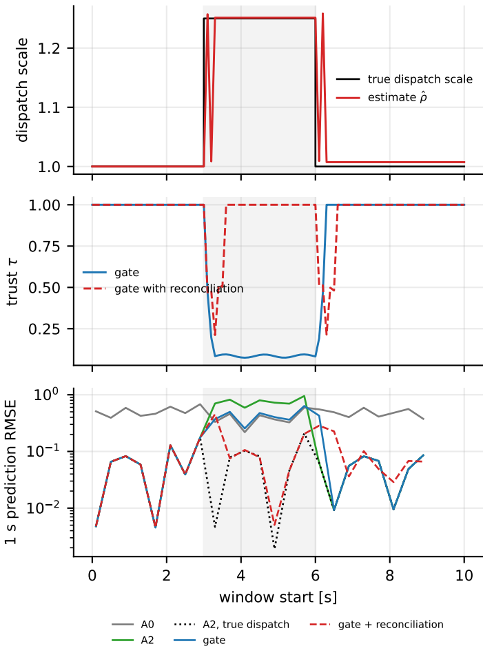
(a) case9: step to \mu = 1.25 at 3 s, undone at 6 s
