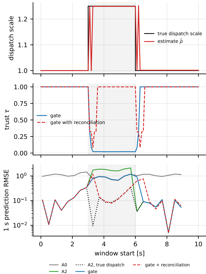
(b) case39: step to \mu = 1.25 at 3 s, undone at 6 s
