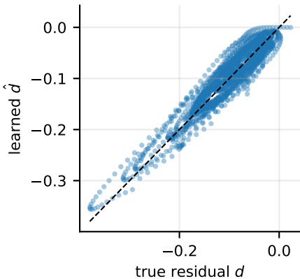
(a) held-out residual
