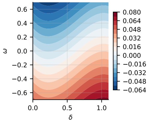
(b) pointwise bound, coverage 0.933
