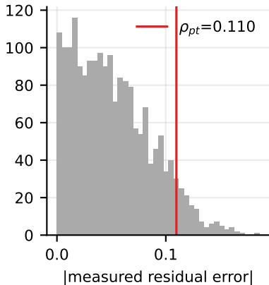
(b) pointwise bound, coverage 0.933
