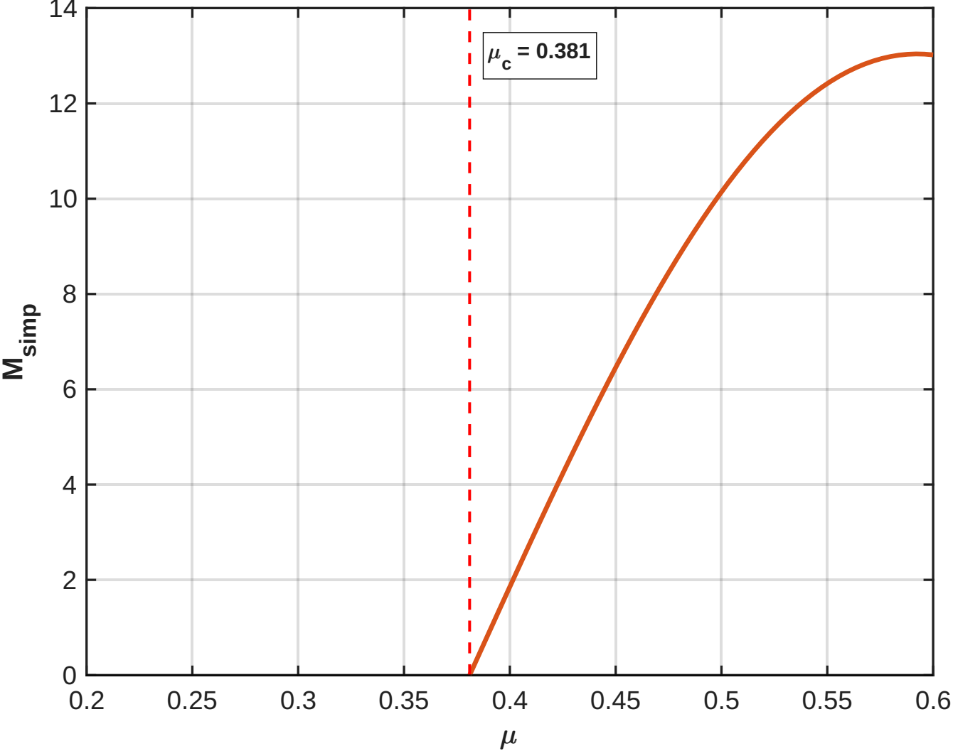
MAPK Cascade 8D Melnikov Function
