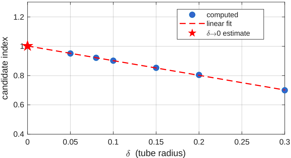
Candidate index vs \delta and its \delta \rightarrow 0 limit
