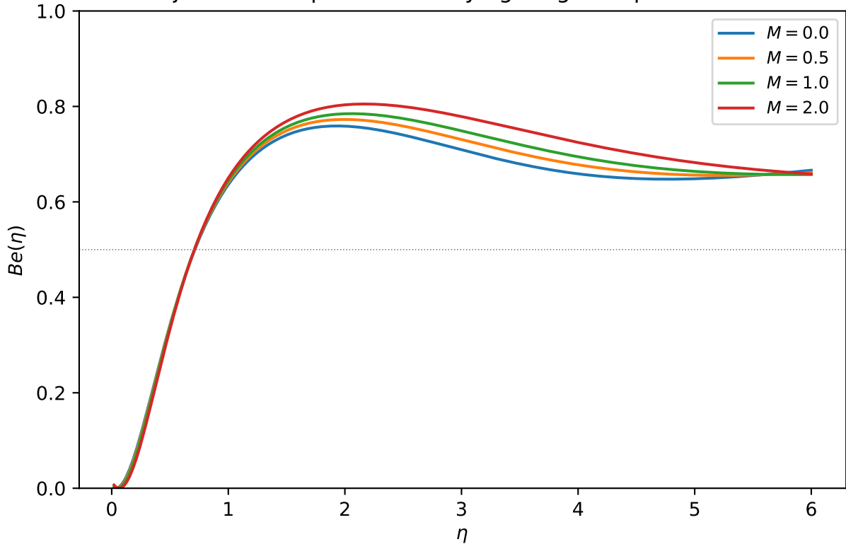
Bejan number profile for varying magnetic parameter M
