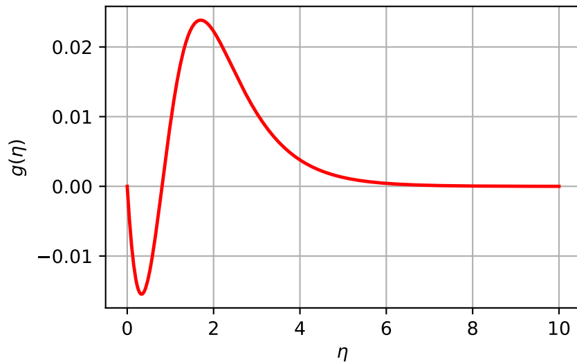
Microrotation profile
