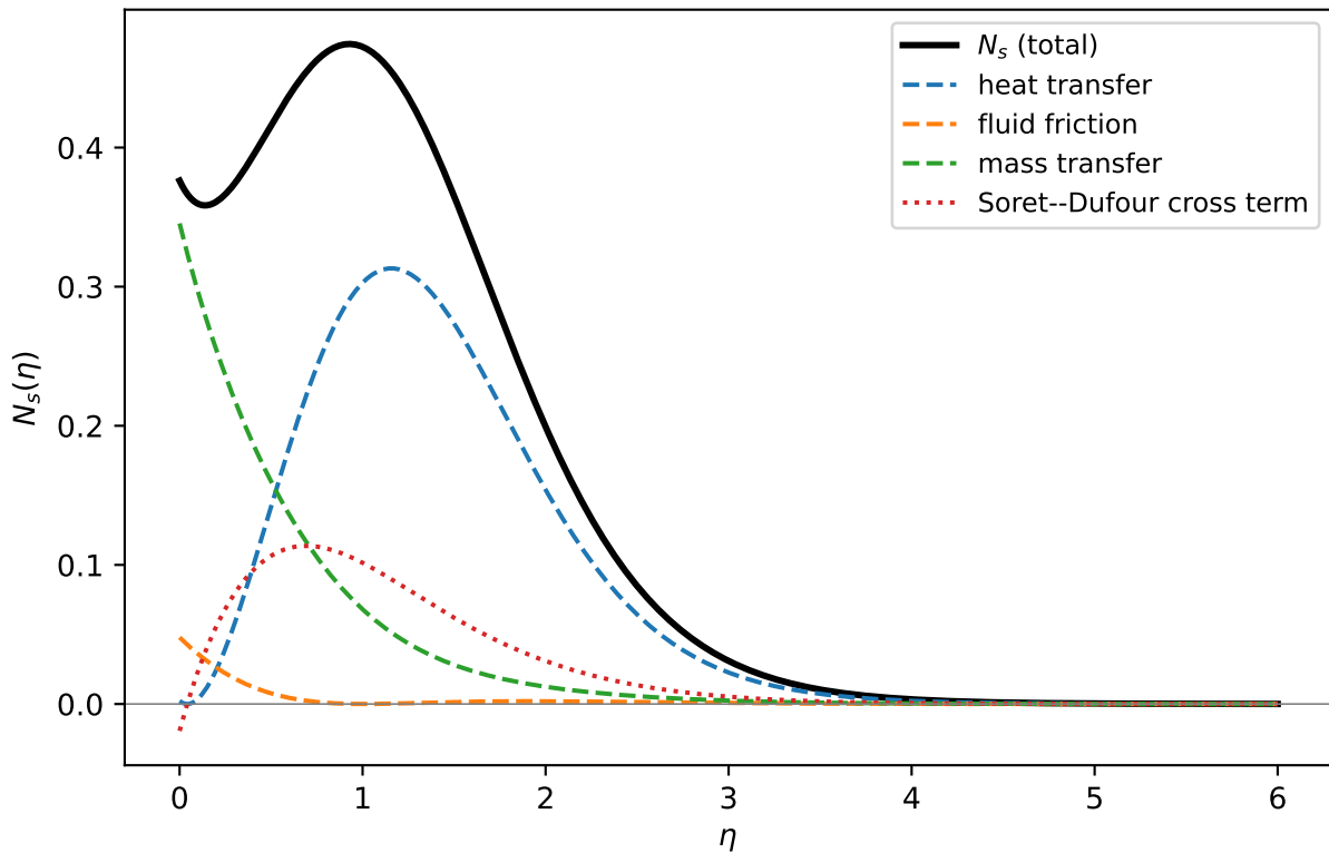
Entropy-generation decomposition at the base parameter set
