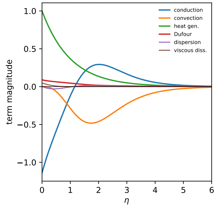
(a) Energy-equation transport budget
