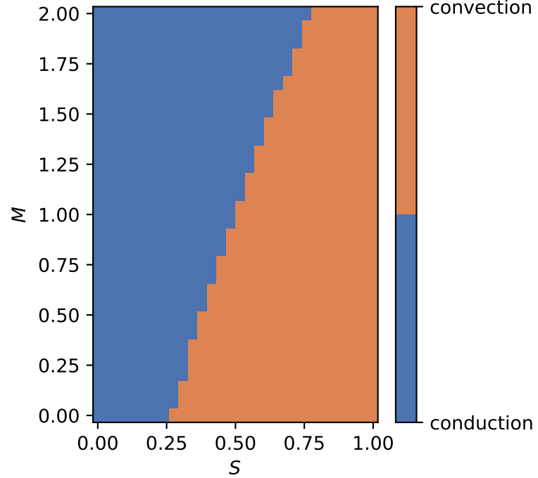
(c) Dominant energy-transport mechanism
