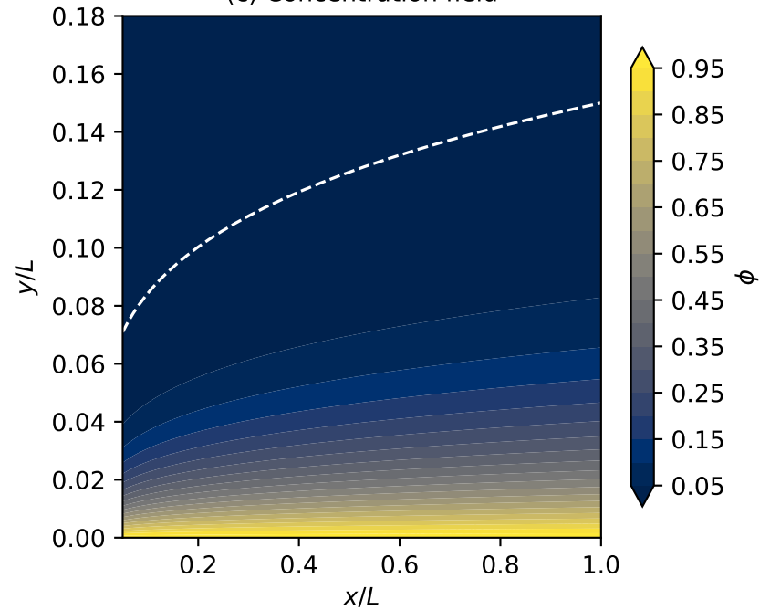
(c) Concentration field
