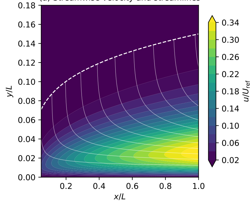
(a) Streamwise velocity and streamlines
