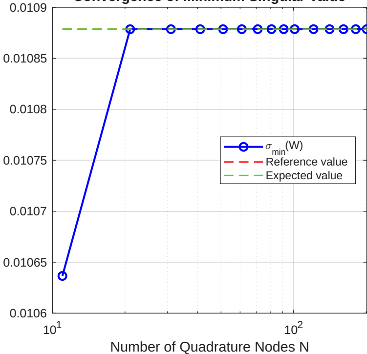
Convergence of Minimum Singular Value
