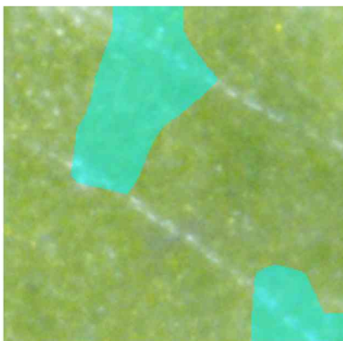
GradCAM
