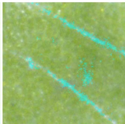
DeepLIFT
