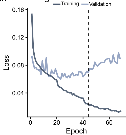
Training and Validation Loss
