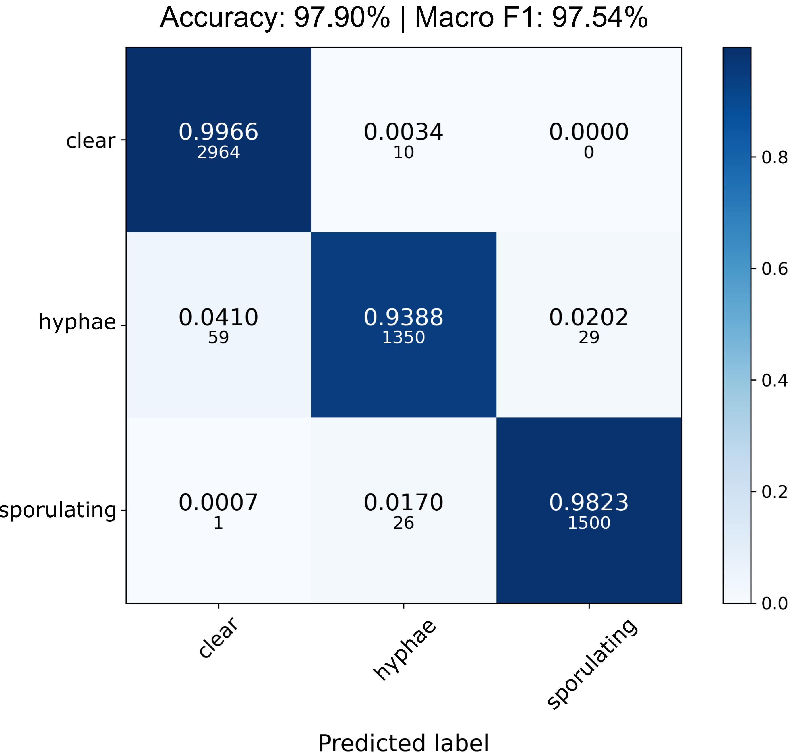
B. Validation, post-optimized thresholds
