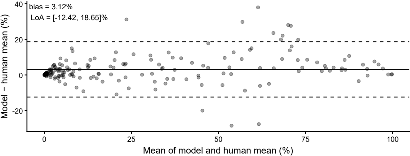
D. Model error tracks rater disagreement
