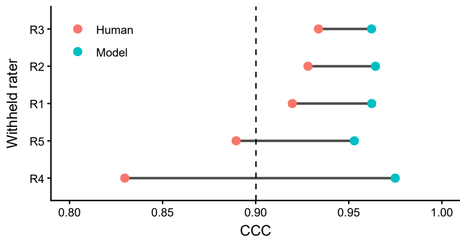
C. LOO concordance vs consensus
