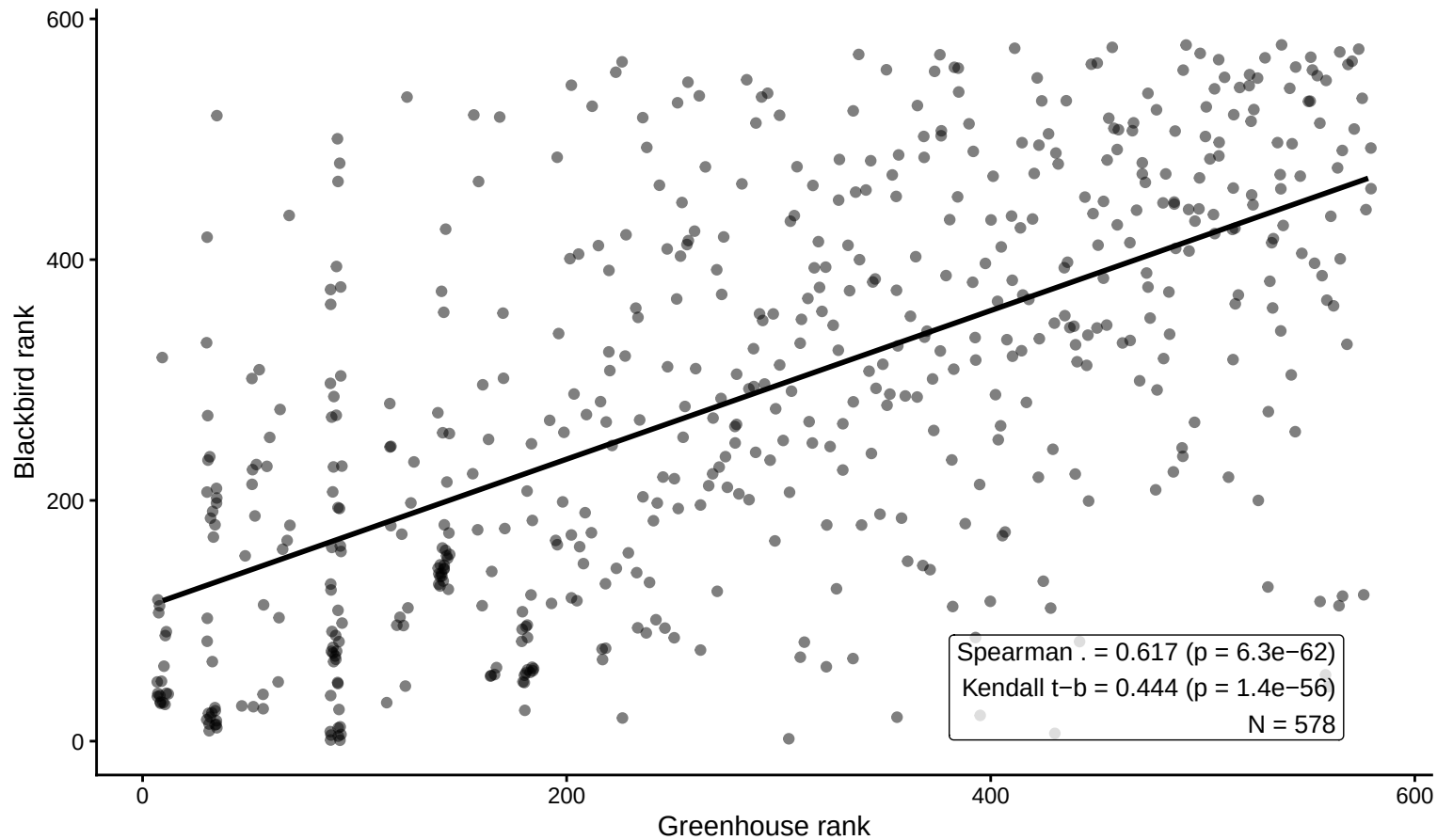
Rank agreement: GH vs Blackbird gradcam_union_sr 10 dpi
