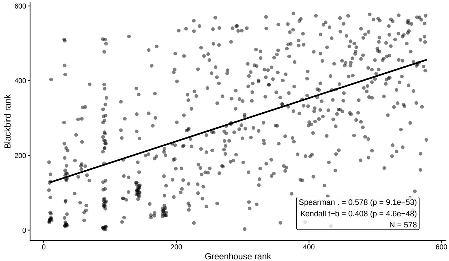
Rank agreement: GH vs Blackbird gradcam 10 dpi
