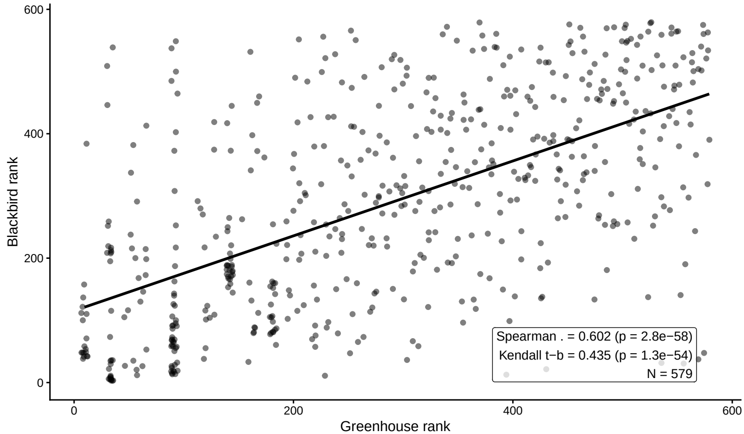
Rank agreement: GH vs Blackbird smoothgrad 5 dpi
