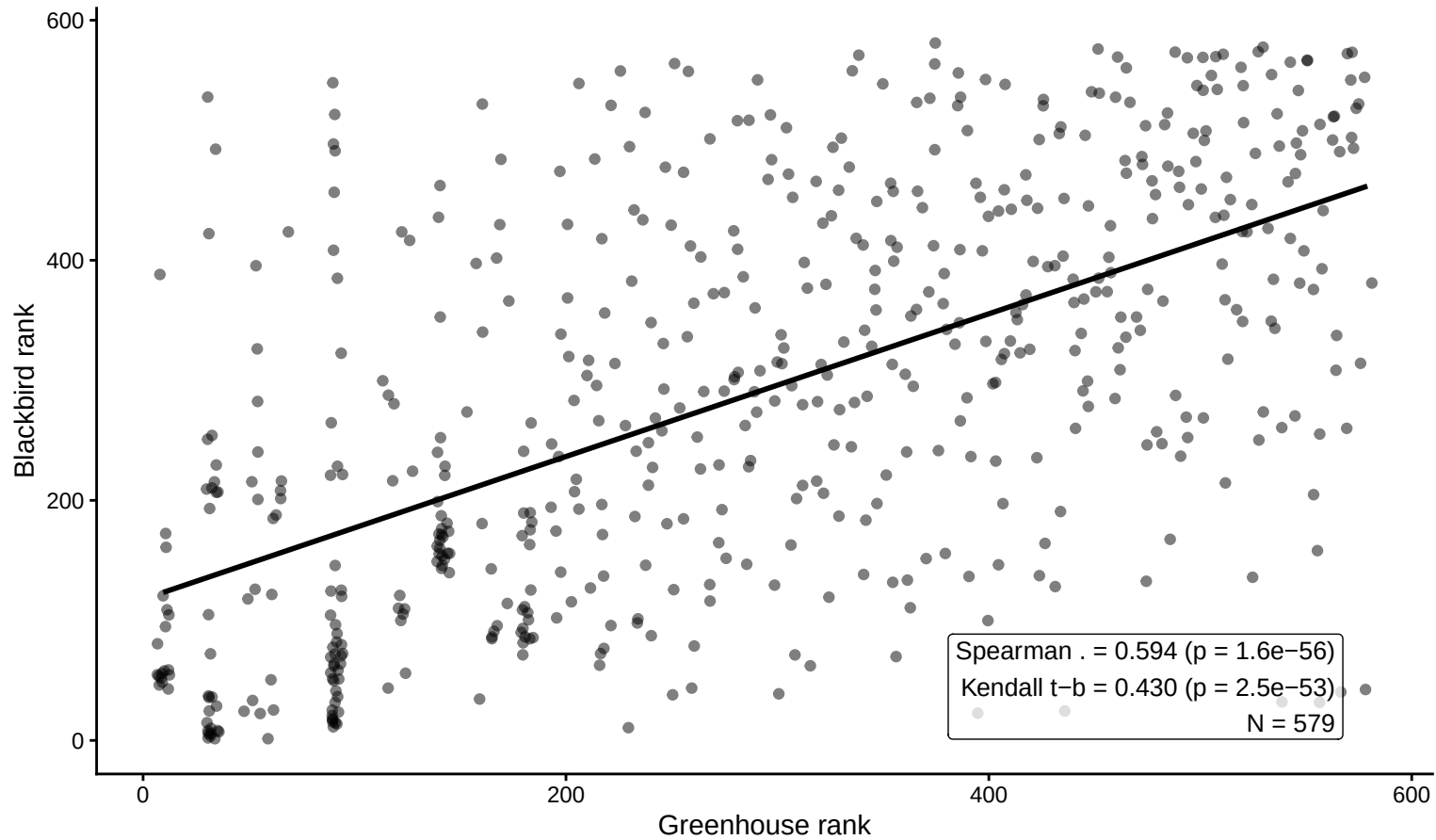
Rank agreement: GH vs Blackbird gradcam_union_sr 5 dpi
