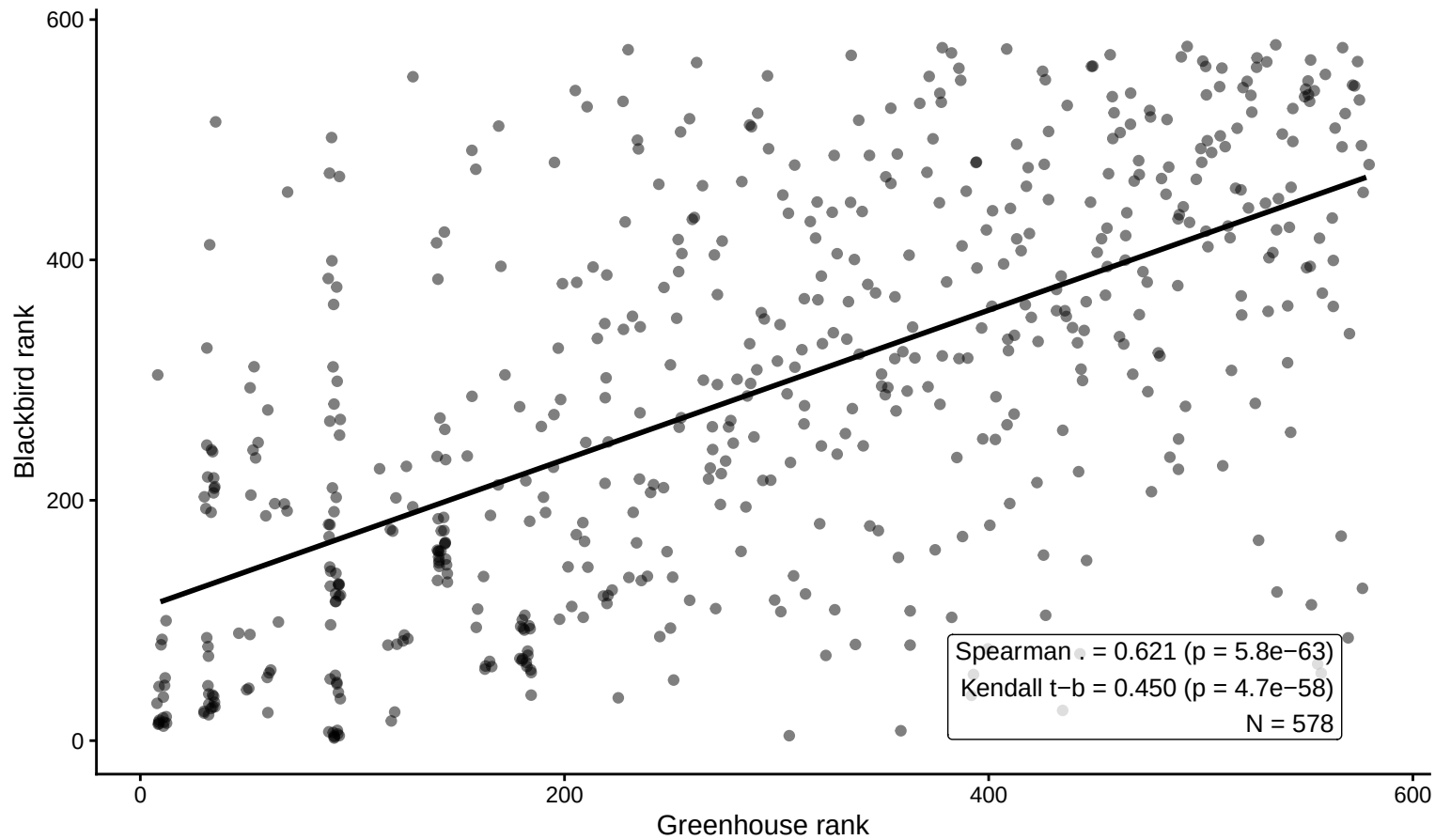
Rank agreement: GH vs Blackbird smoothgrad_union_sr 10 dpi
