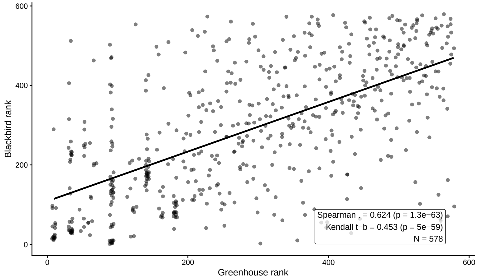
Rank agreement: GH vs Blackbird smoothgrad_spor_sr 10 dpi
