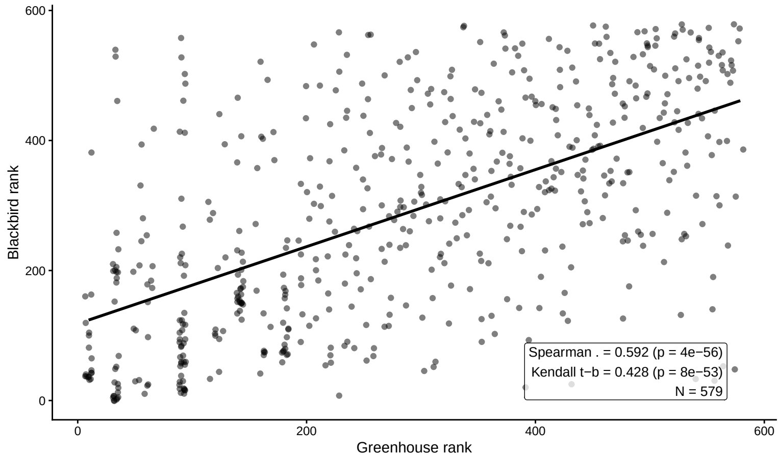
Rank agreement: GH vs Blackbird gradcam_inf_sr 5 dpi
