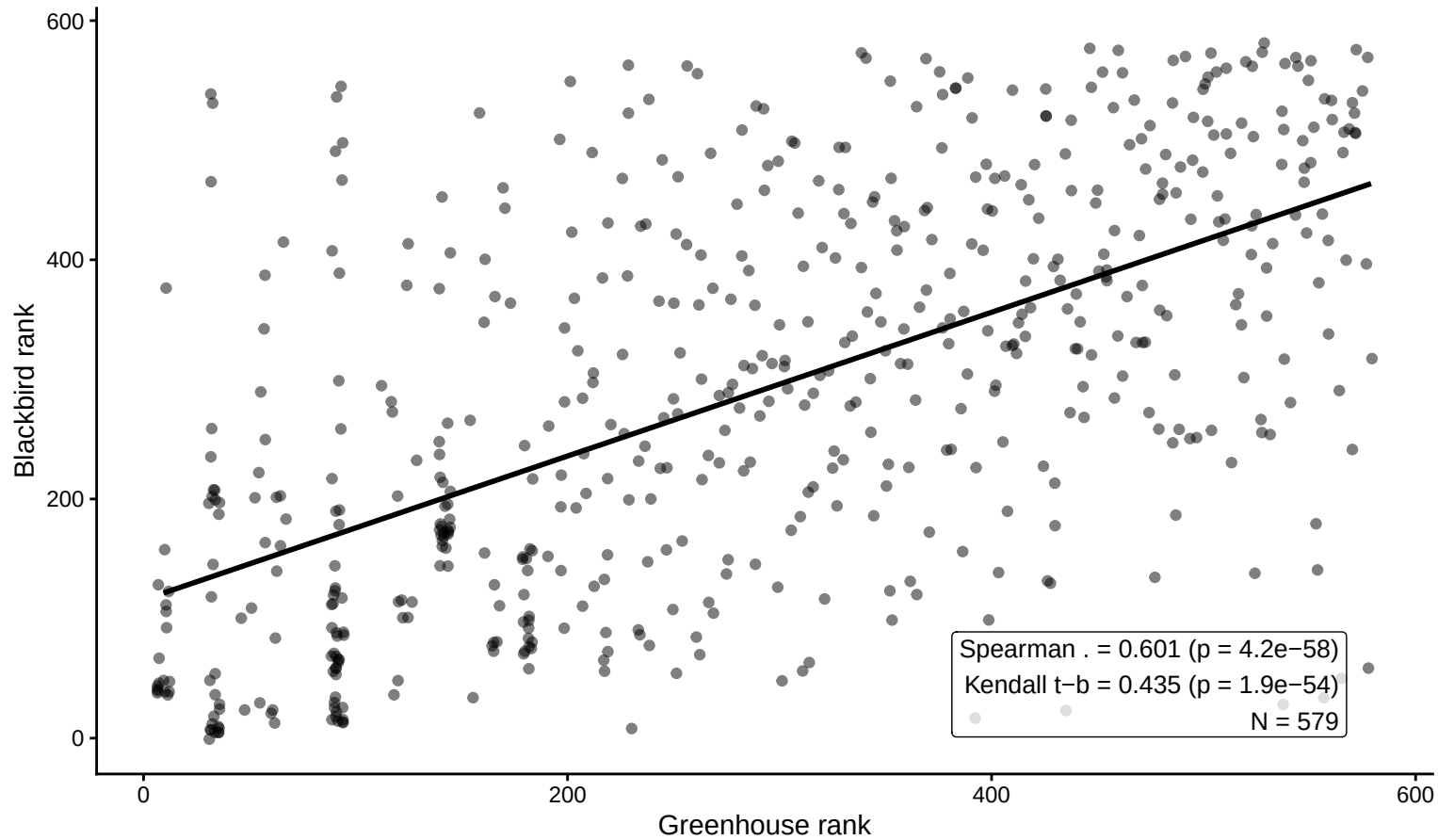
Rank agreement: GH vs Blackbird smoothgrad_inf_sr 5 dpi
