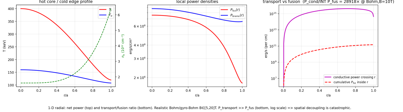
Representative decoupled profile (Wang, T_{i,core}=400 keV, \kappa_T=0.3 , Bohm \chi , B=10 T)
