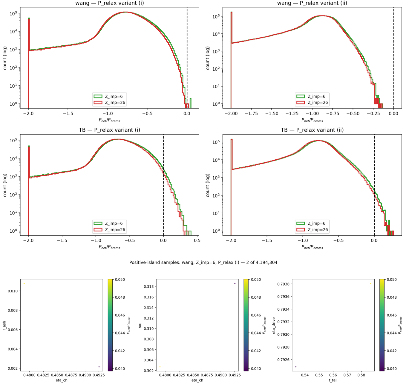
FIG. 3. Combinatorial net-power scan ( 4.19 \times 10^6 Sobol samples, seven free levers). Left: distribution of P_{\text{net}}/P_{\text{brems}} for the two cross sections and the two recirculation-accounting variants, with the ignition threshold marked; the strict-accounting Wang distribution lies entirely below threshold. Right: parameter projection of the rare positive samples.
