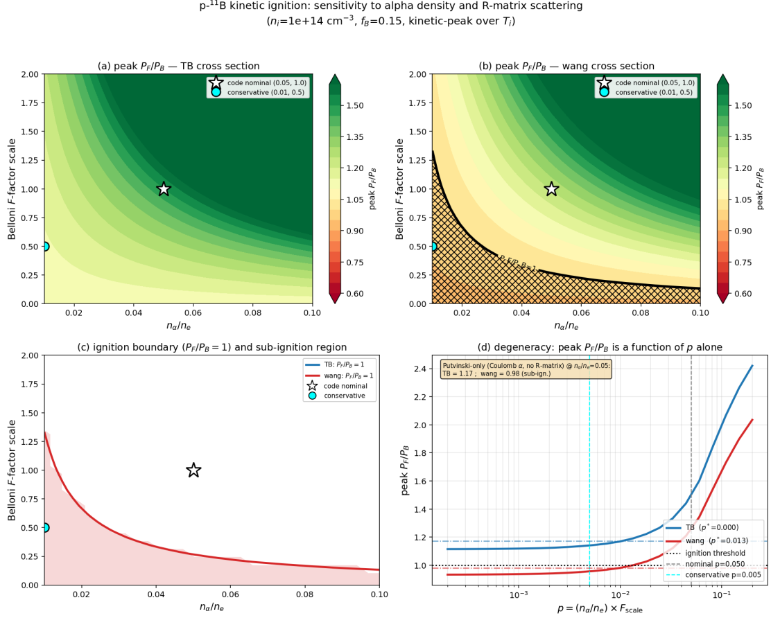
FIG. 2. Two-dimensional kinetic-uncertainty map. Because the enhancement depends only on p = (n_\alpha/n_e) \cdot F_{\text{scale}} , the ignition boundary is a hyperbola; the panel shows peak P_F/P_B over the (n_\alpha, F_{\text{scale}}) plane for both cross sections, with the P_F/P_B = 1 contour, the defensible channeling-efficiency limit, and the Putvinski-only (no-R-matrix) reference.
